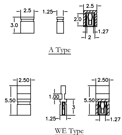
2206-Series 1.27mm(0.050")
