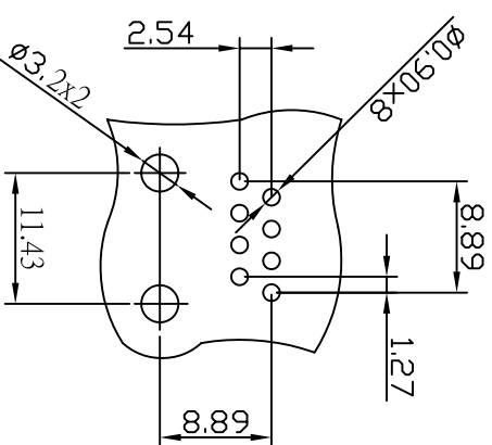
LAYOUT/TOP VIEW
