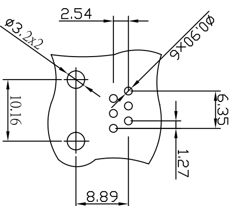
LAYOUT/TOP VIEW
