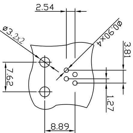
LAYOUT/TOP VIEW
